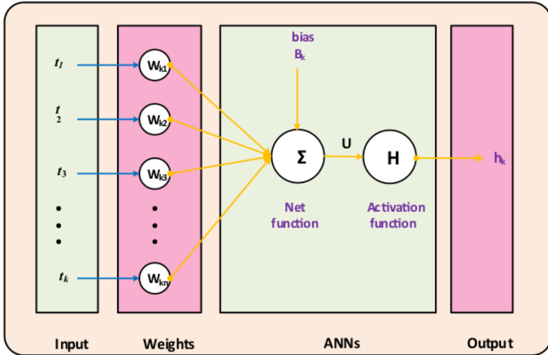
Fig. 2 Single neuron structure
