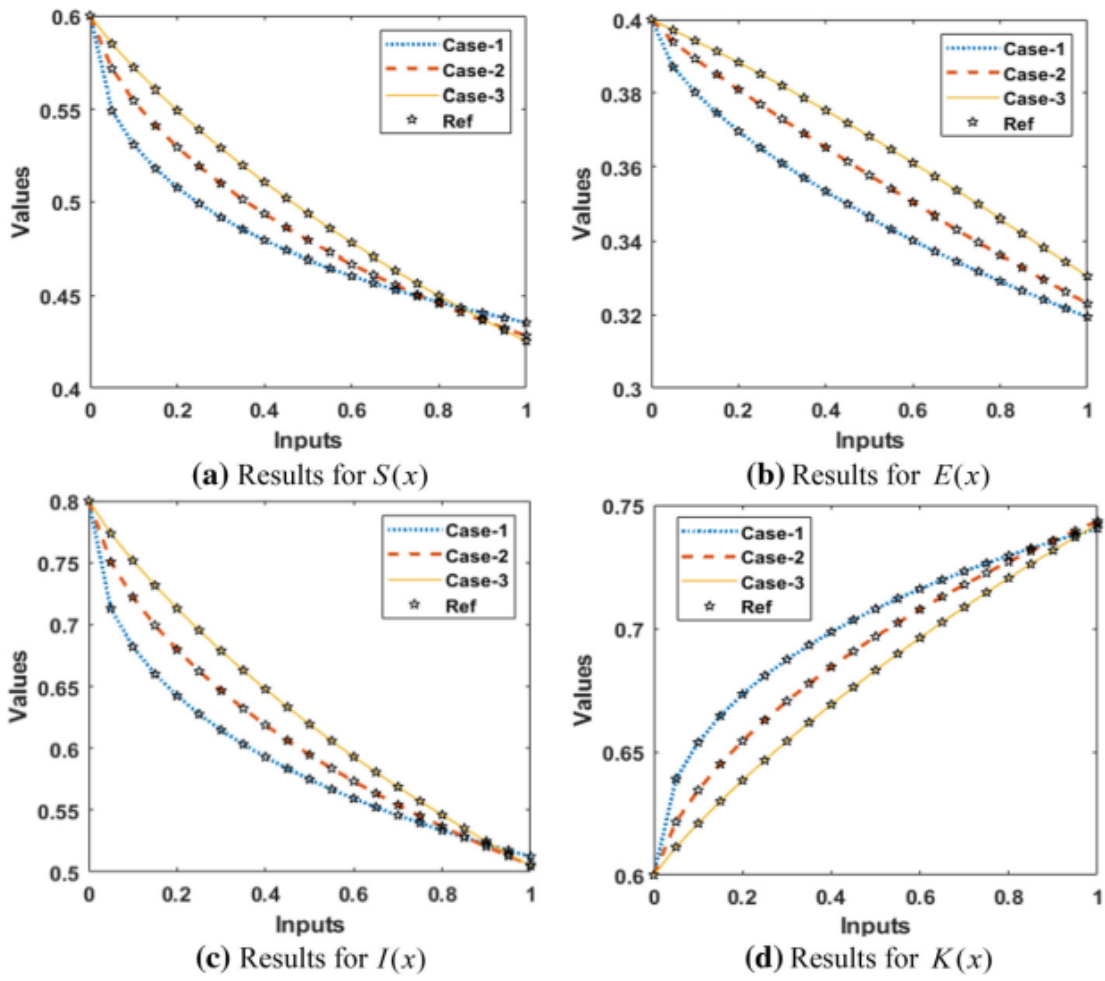
8 Fig. 7 Comparison of the result to solve the FO-SEIR-KS mathematical model
