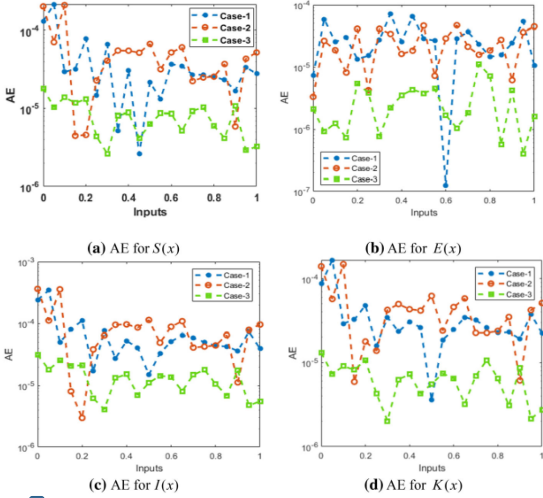
8 Fig. 8 AE to solve the FO-SEIR-KS mathematical model
