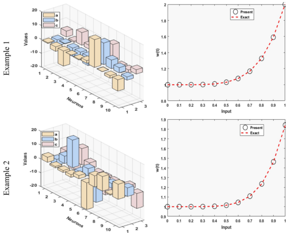
10 Fig. 2 Set of weights and comparison of exact/proposed results for both the examples of fifth-order LE model of type 1
