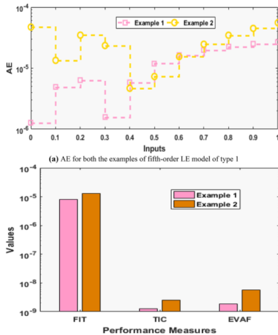
4 Fig. 3 AE and performance gages for both the examples of fifth-order LE model of type 1
