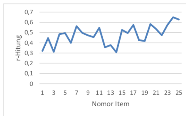
Figure 1. r_{count} Value of Each Item
